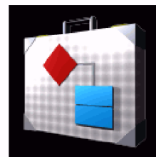
ReadAppsXML functions
